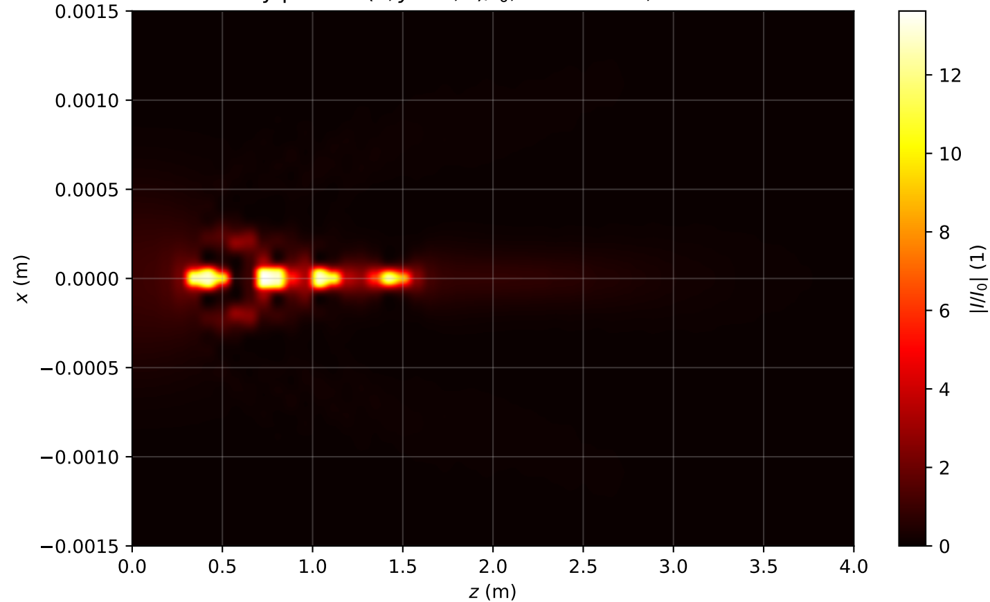
Intensity profile I(x, y = 0, z)/I_0 , P_{in}=8.5P_{cr} , artificial time
